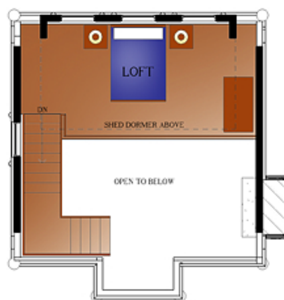
LOFT FLOOR
